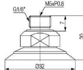
[ With M518MFX fitting ]
