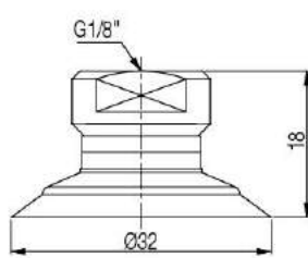
[ With 18F fitting ]
